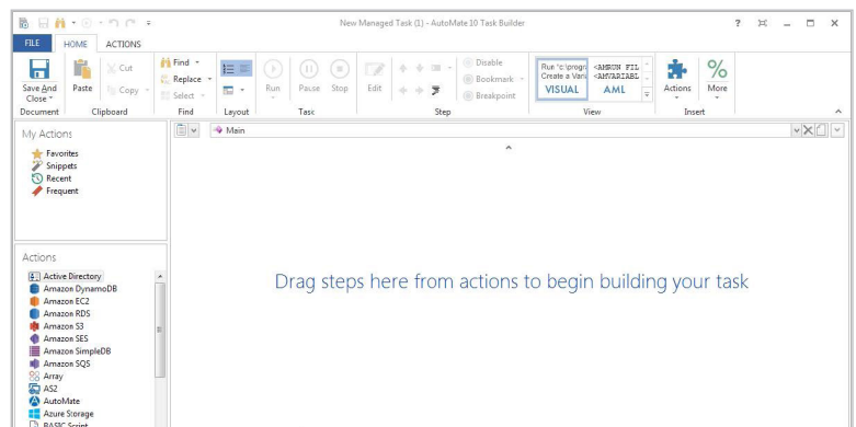
Automate Enterprise Server's Task Builder provides an easy, no-code platform for building even the most complex tasks.
